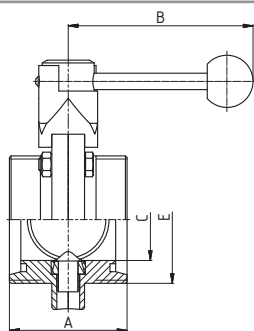
Butterfly valve G - G Scheibenventil G - G
